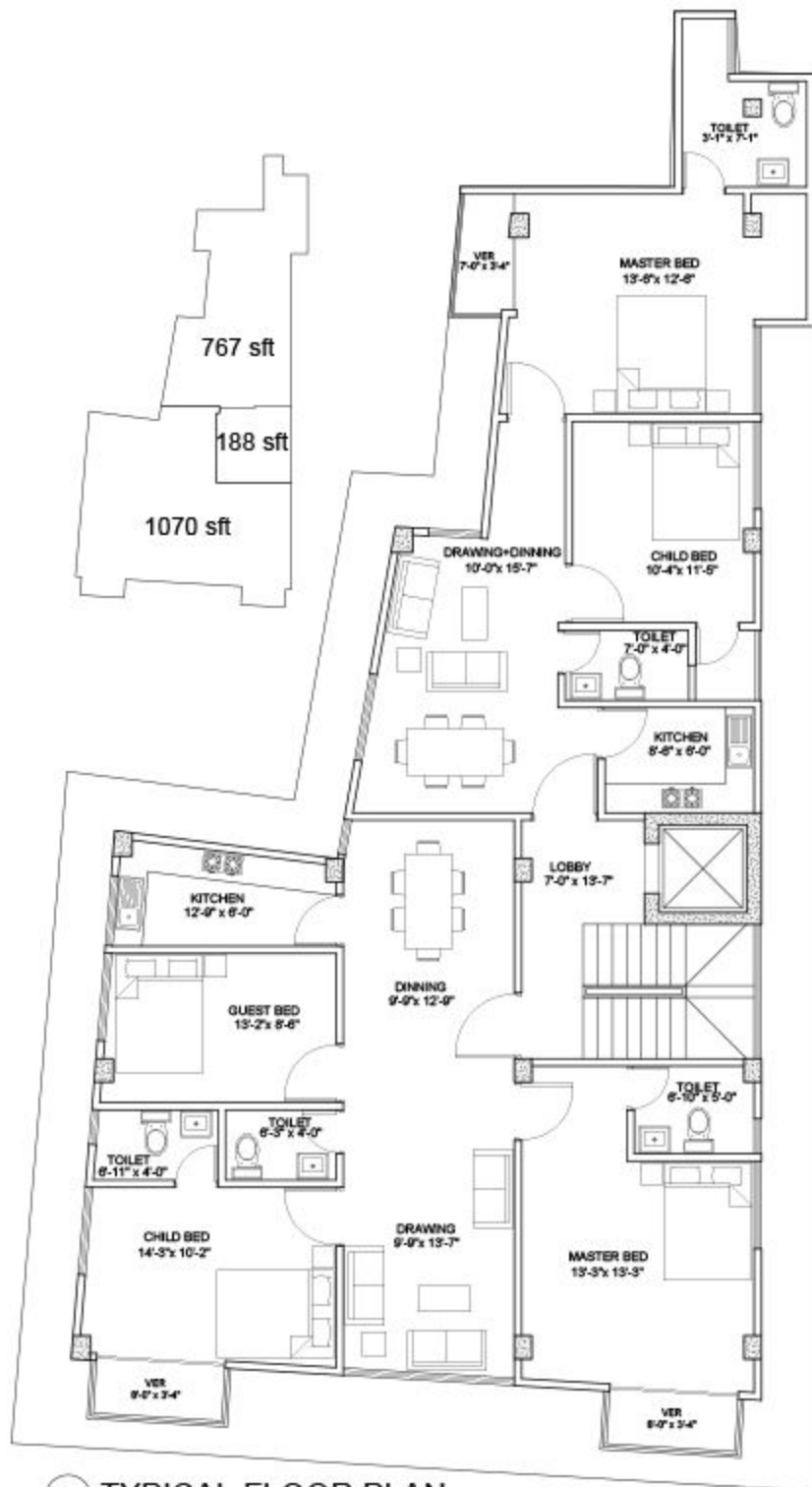
1 TYPICAL FLOOR PLAN
